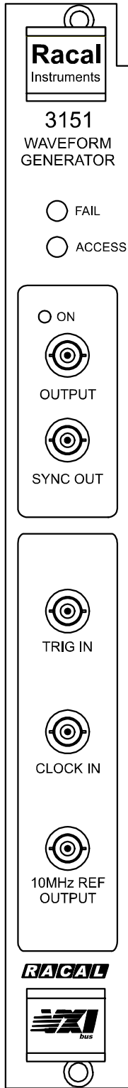
Figure 1-1, 3151A+ Front Panel
