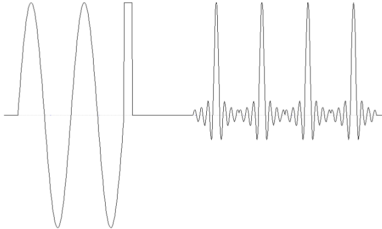
Figure 3-6, Sequenced Waveforms - Continuous Advance Mode
