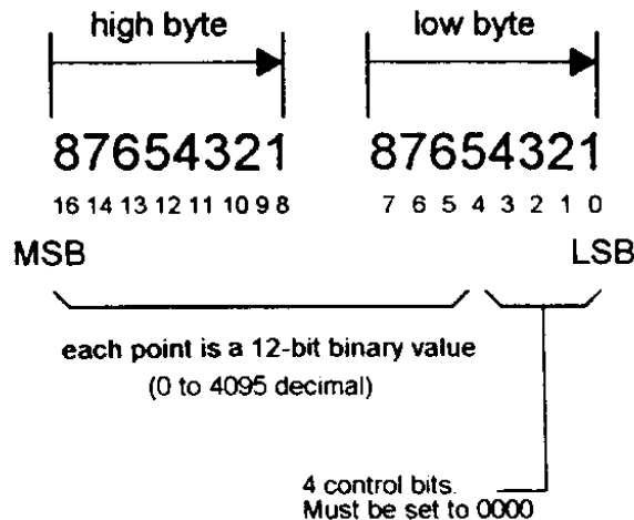
Figure 3-2 12-Bit Waveform Data Format
