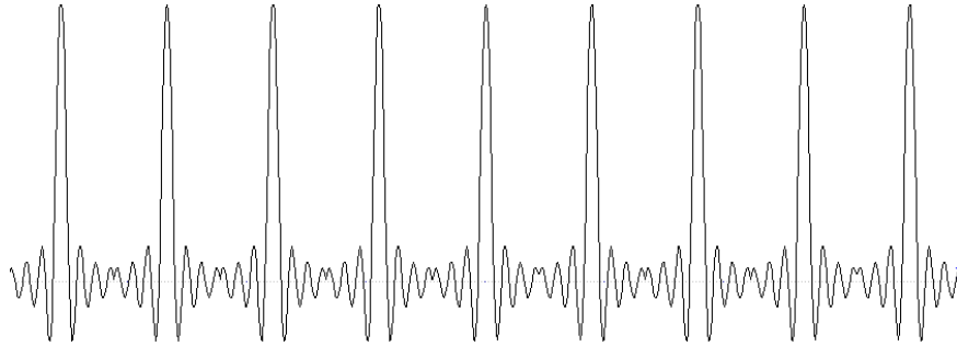
Figure 3-3, Sin(x)/x Waveform Loaded Into Segment 1
